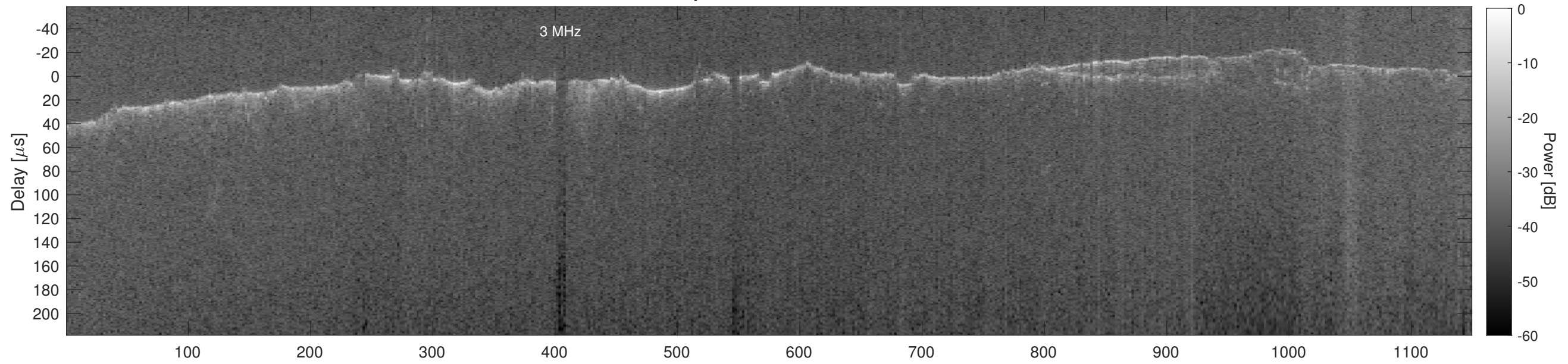
Orbit 15219, Cluttergram
