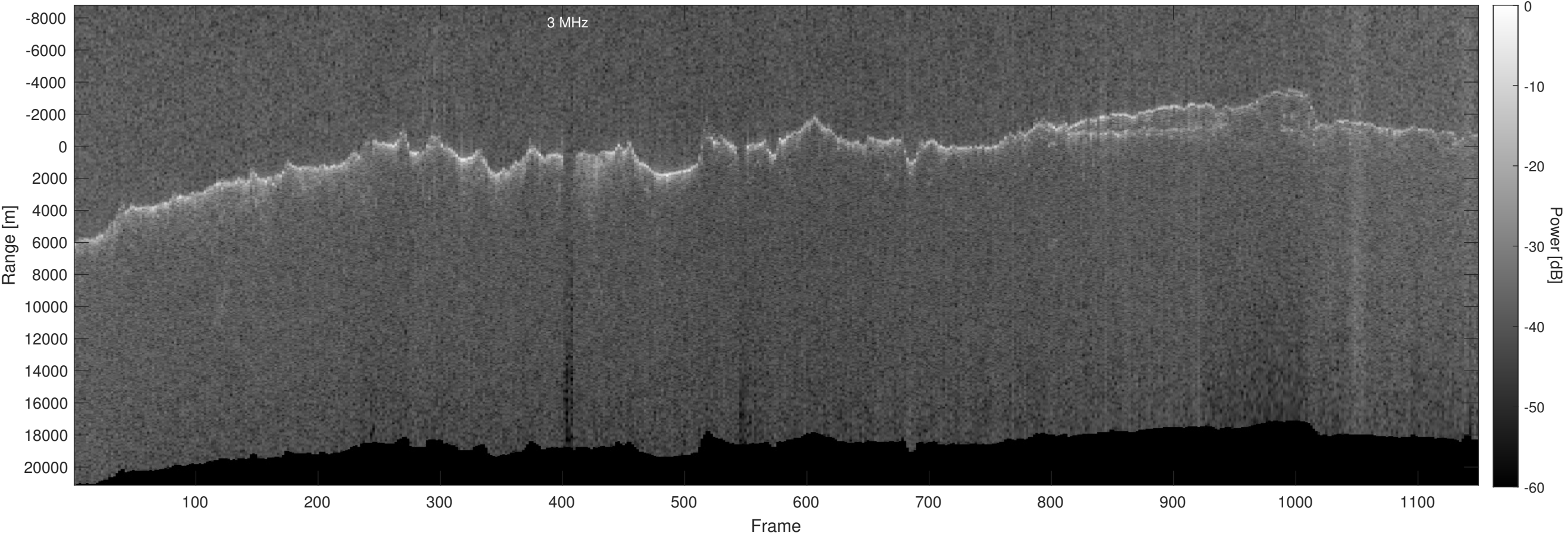
Orbit 15219, Optimized, No Window, Depth-Corrected, Channel 2
