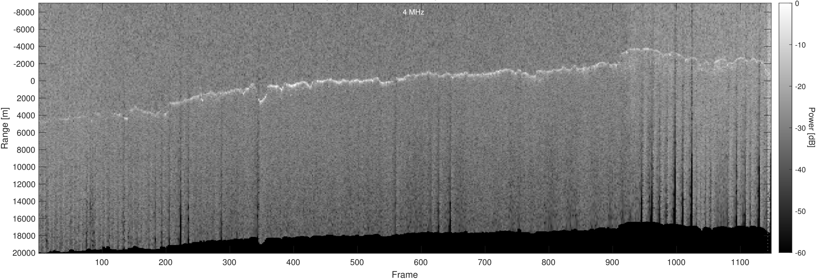
Orbit 15221, Optimized, No Window, Depth-Corrected, Channel 2
