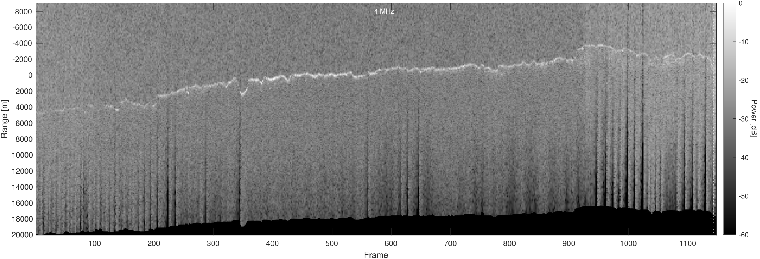
Orbit 15221, Optimized, Window, Depth-Corrected, Channel 2
