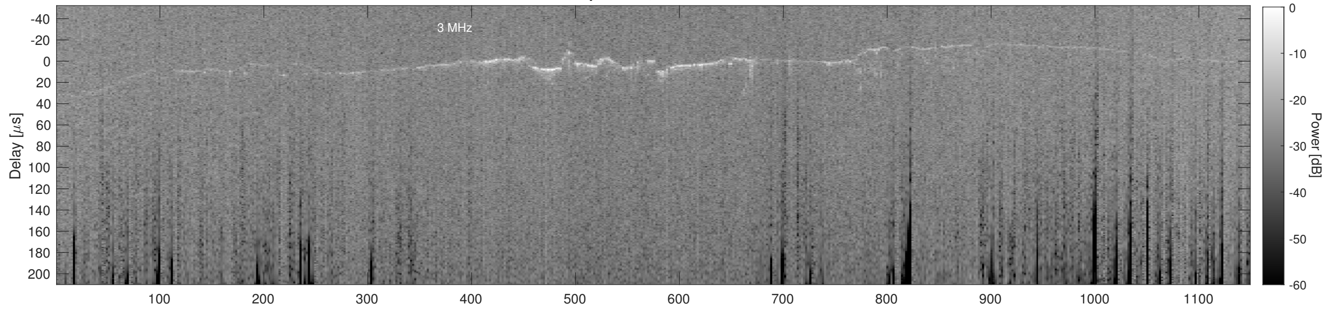
Orbit 15223, Cluttergram
