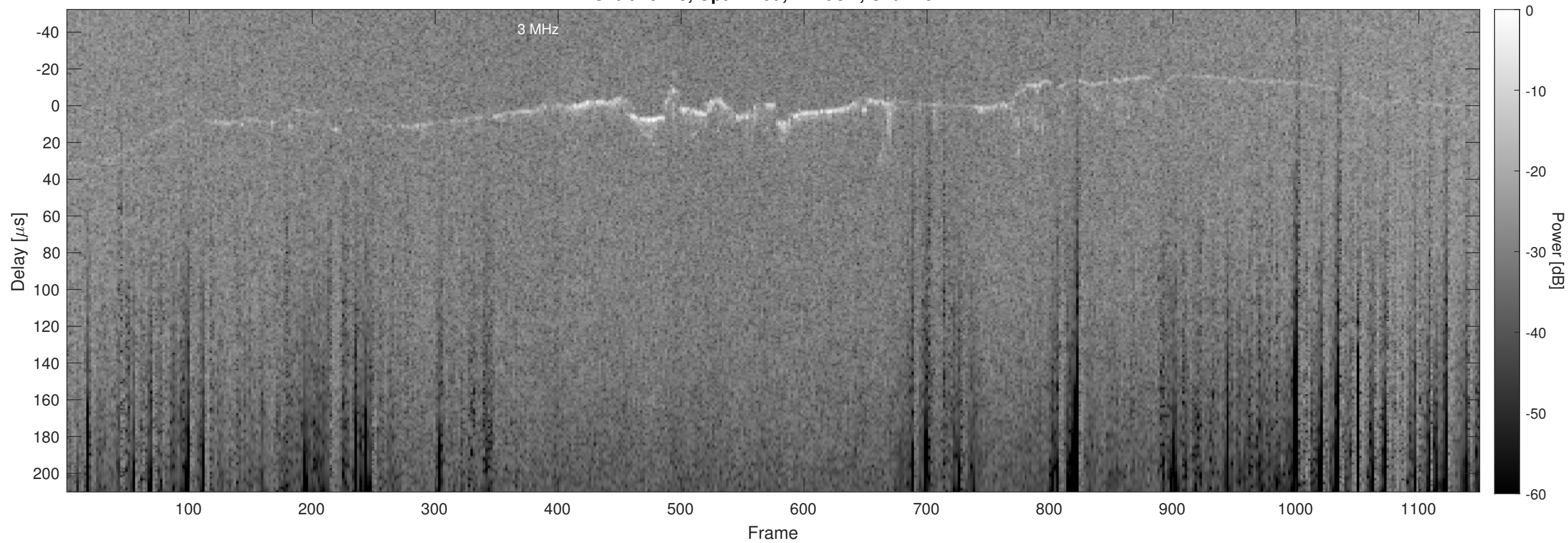
Orbit 15223, Optimized, Window, Channel 2
