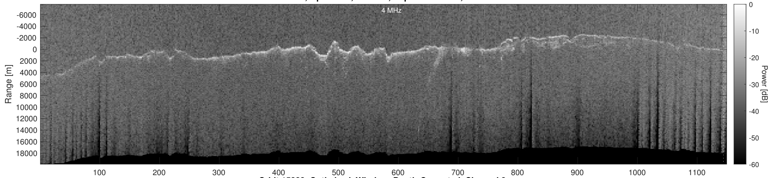
Orbit 15223, Optimized, Window, Depth-Corrected, Channel 2
