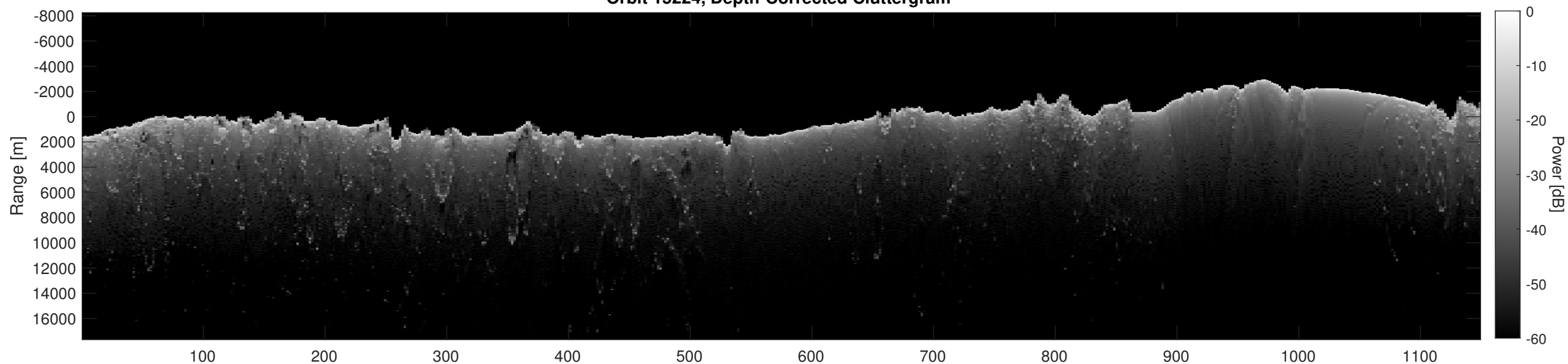
Orbit 15224, Depth-Corrected Cluttergram
