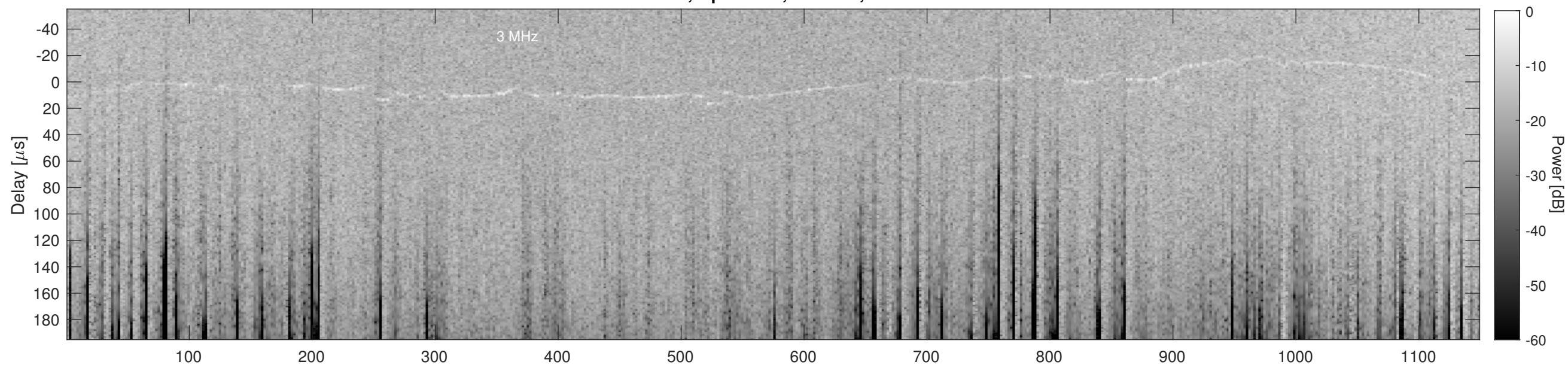
Orbit 15224, Cluttergram
