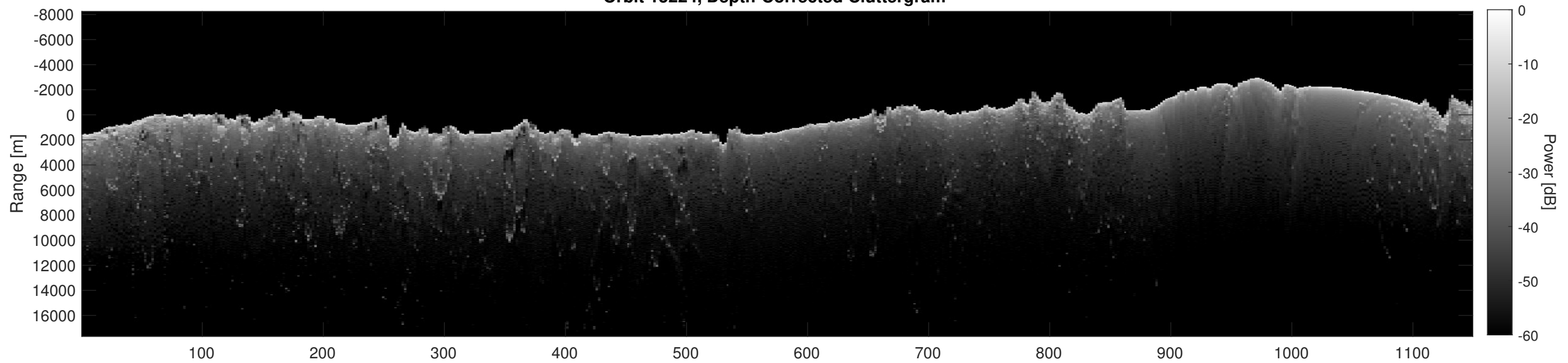
Orbit 15224, Depth-Corrected Cluttergram
