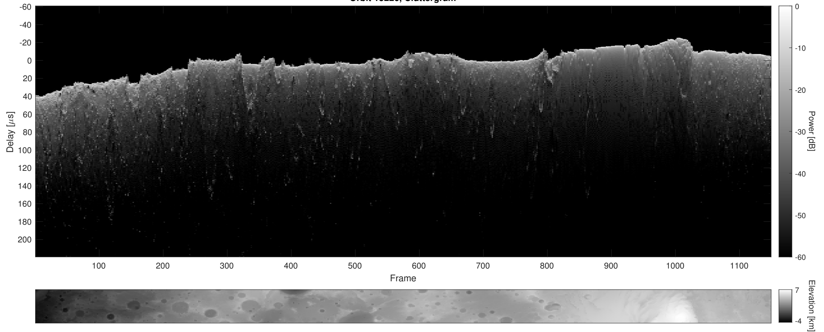
Orbit 15226, Cluttergram
