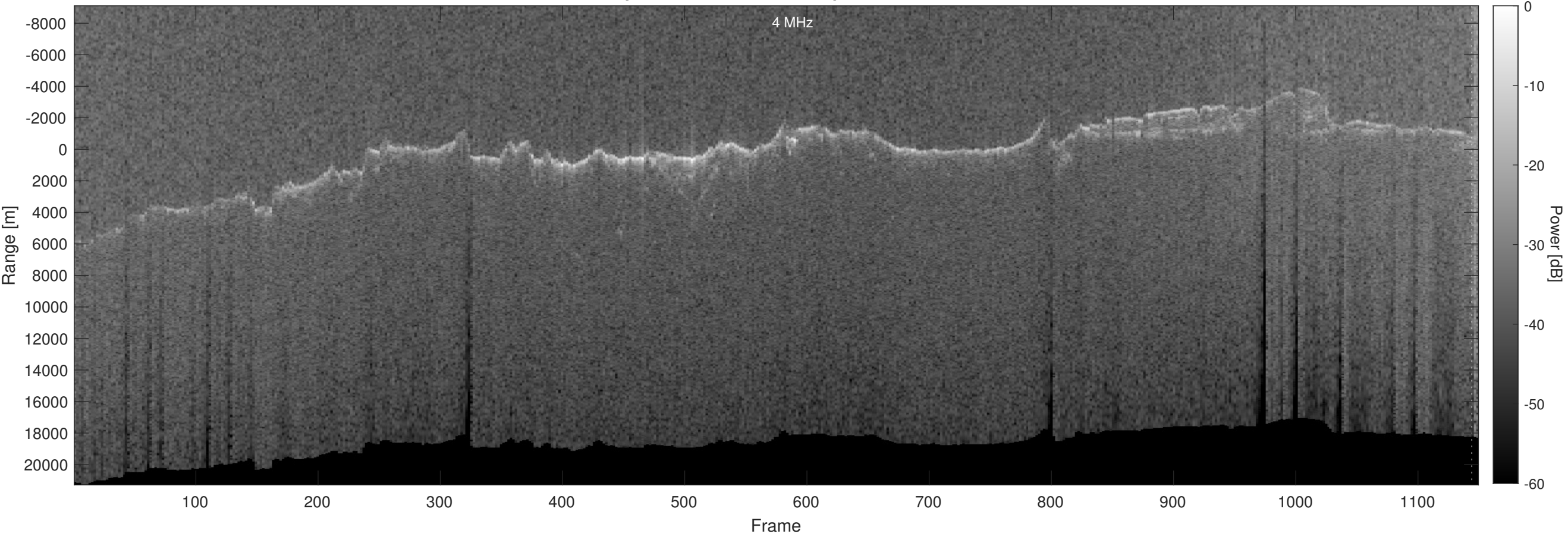
Orbit 15226, Optimized, No Window, Depth-Corrected, Channel 2
