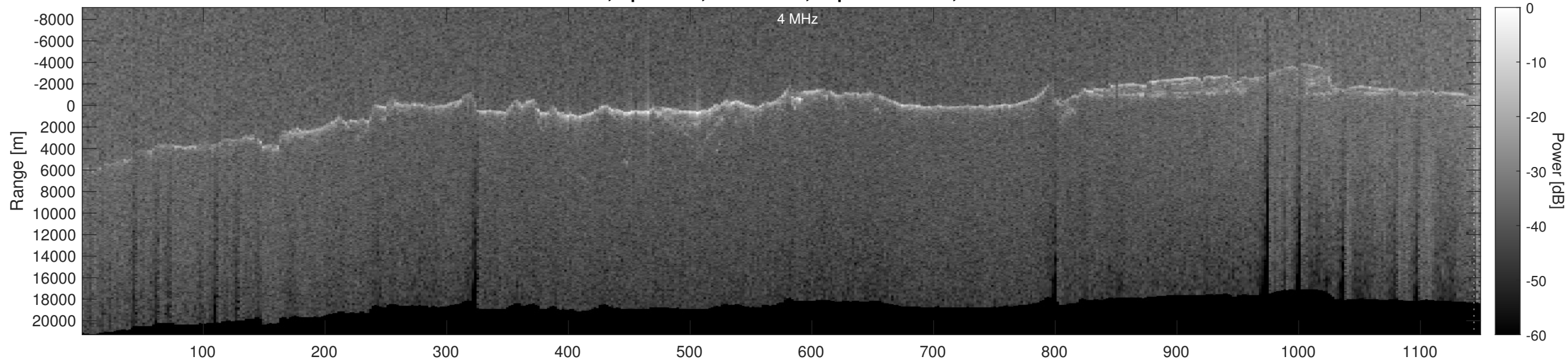
Orbit 15226, Optimized, No Window, Depth-Corrected, Channel 2
