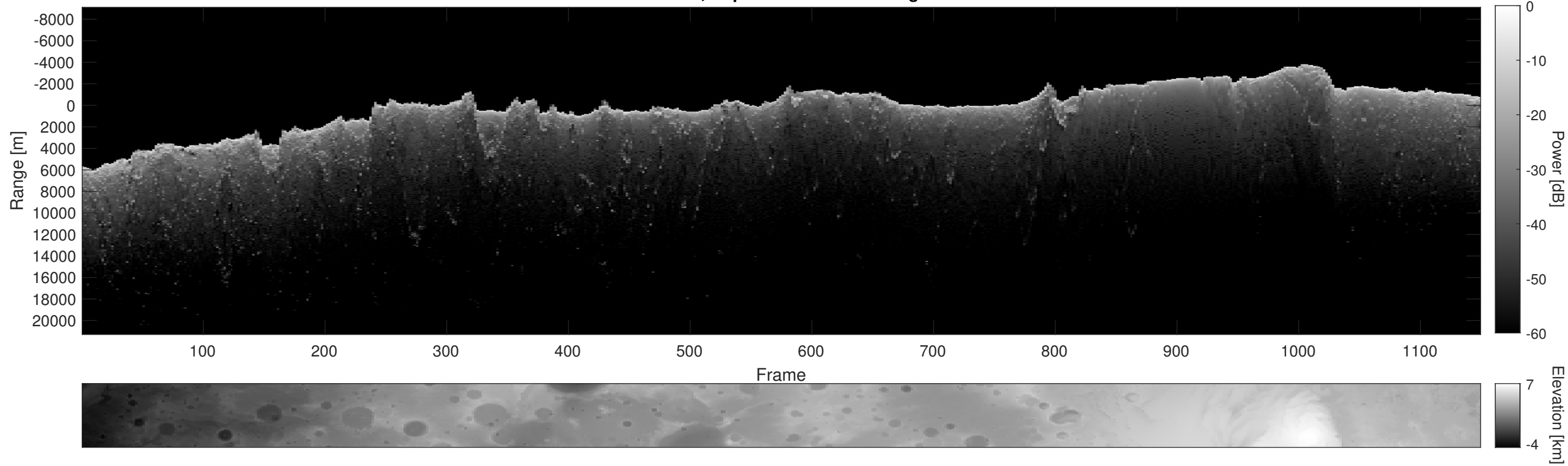
Orbit 15226, Depth-Corrected Cluttergram
