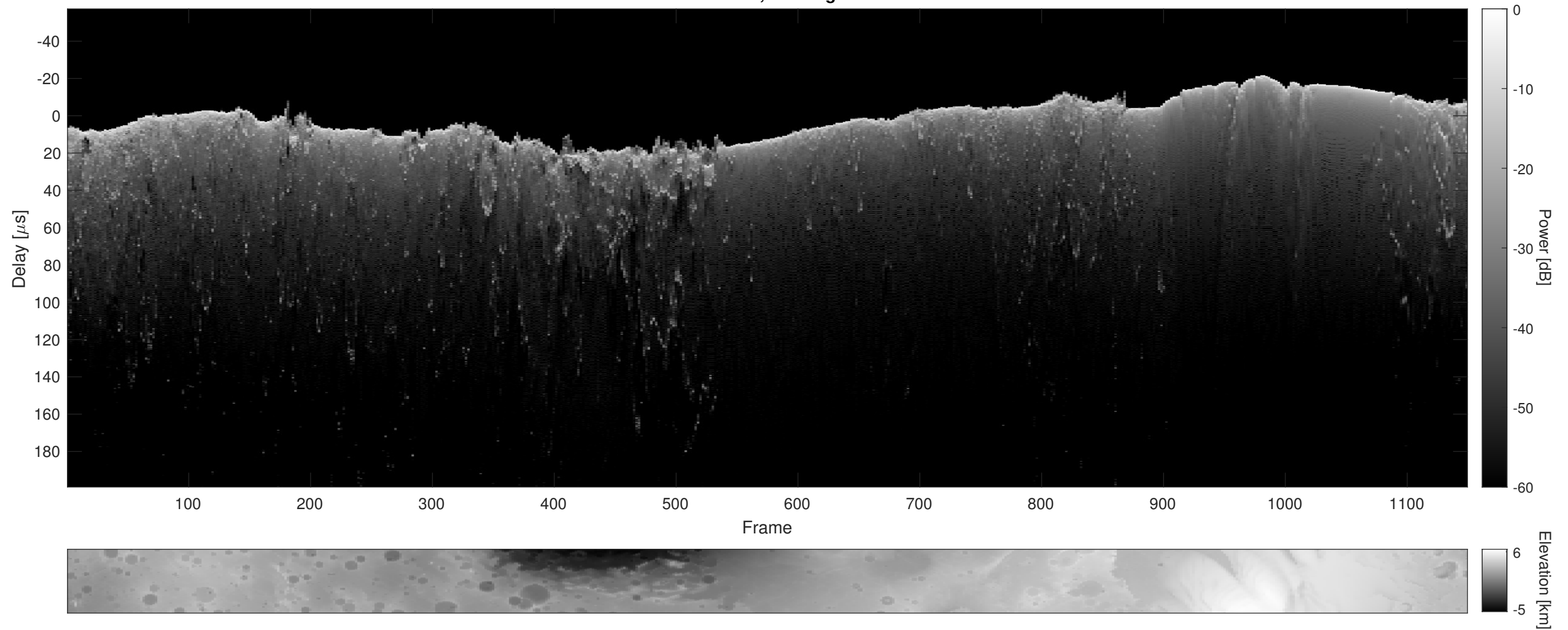
Orbit 15231, Cluttergram
