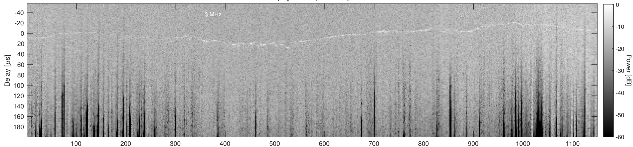
Orbit 15231, Cluttergram
