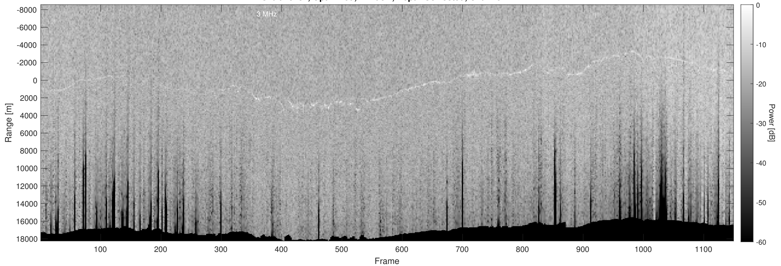
Orbit 15231, Optimized, Window, Depth-Corrected, Channel 2
