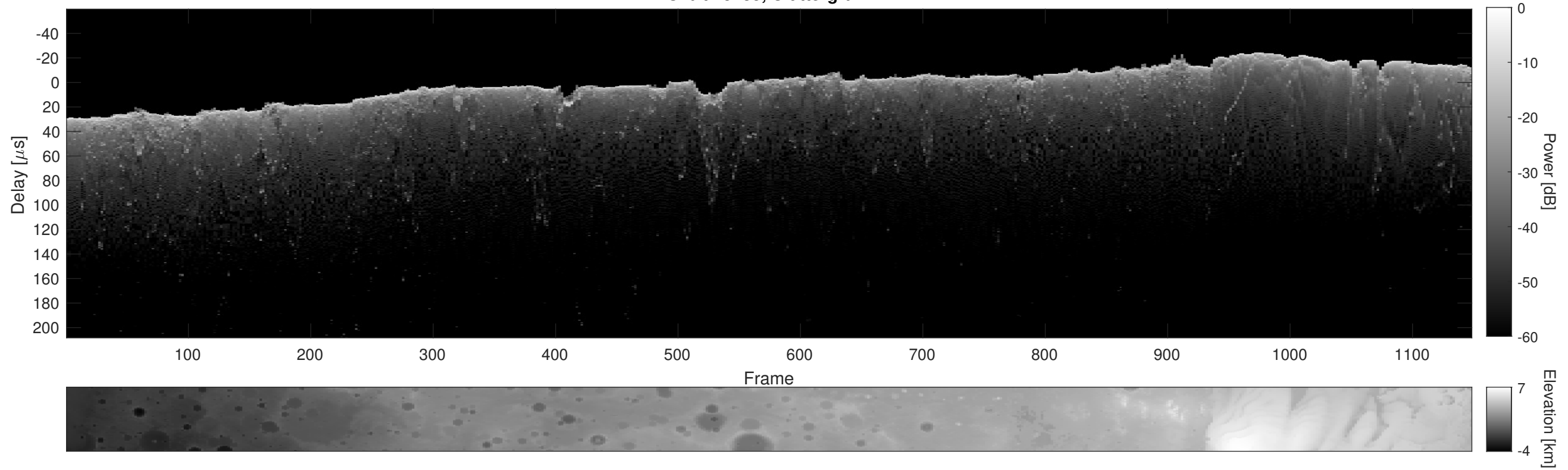
Orbit 15235, Cluttergram
