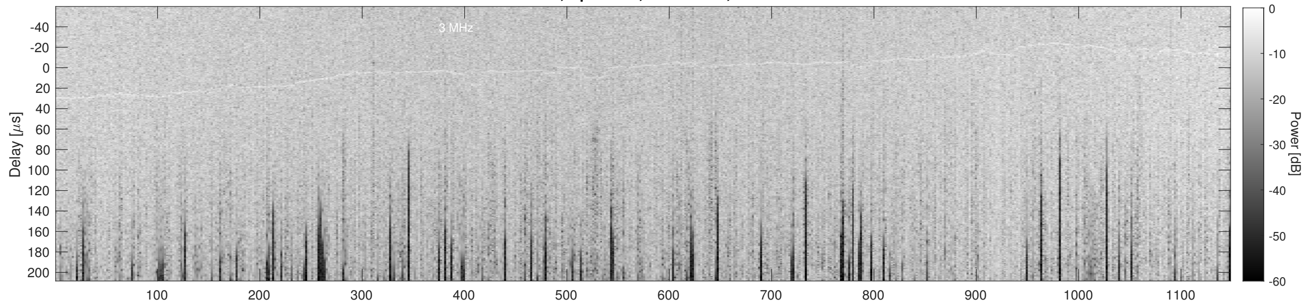
Orbit 15235, Cluttergram
