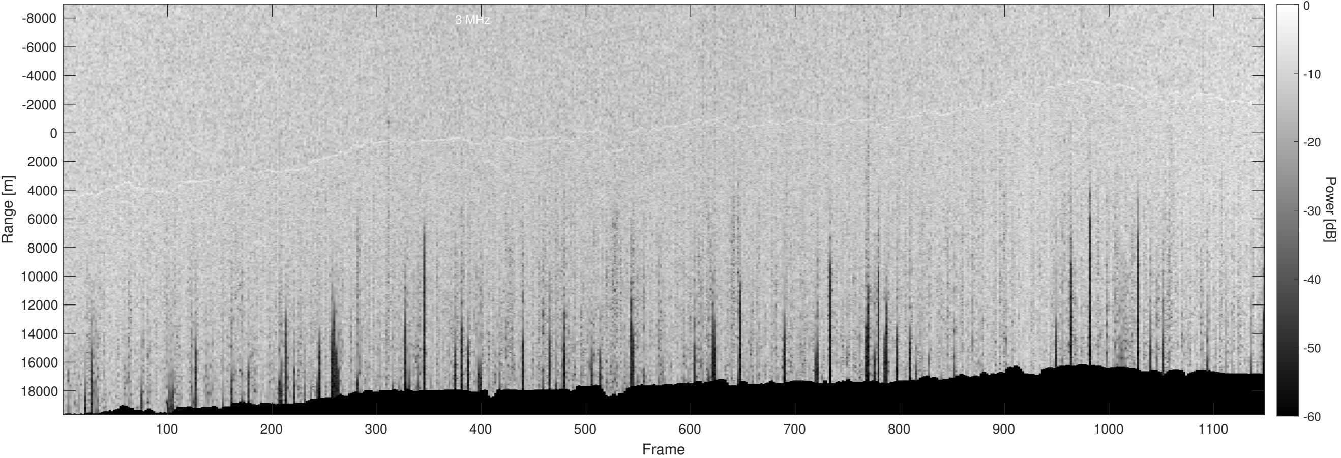
Orbit 15235, Optimized, No Window, Depth-Corrected, Channel 2
