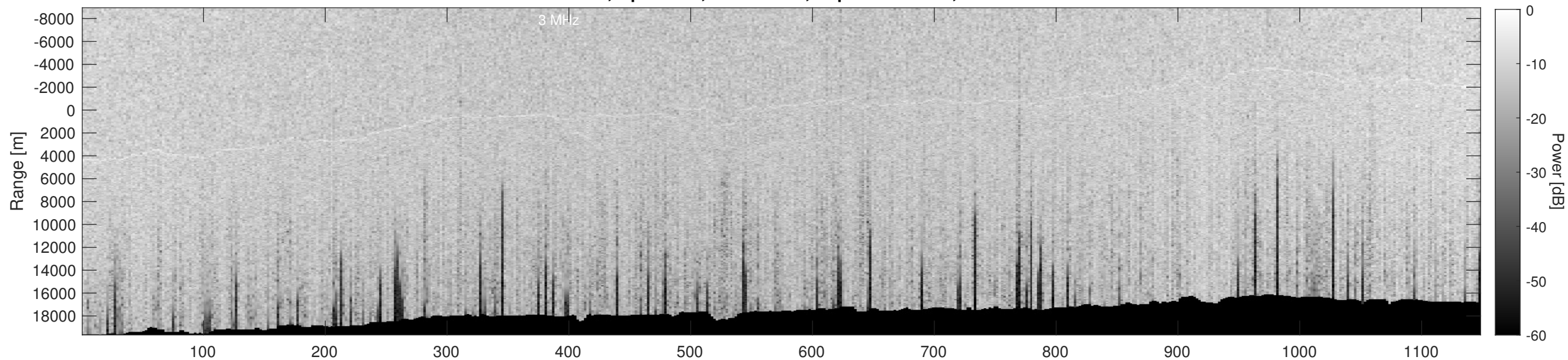
Orbit 15235, Depth-Corrected Cluttergram
