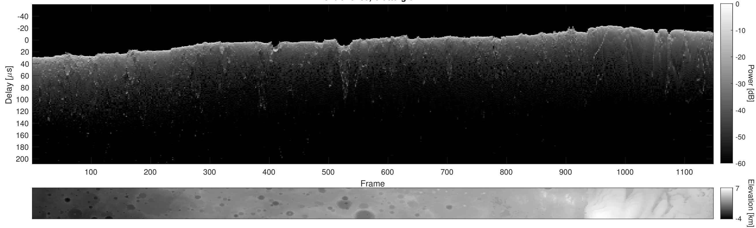
Orbit 15235, Cluttergram
