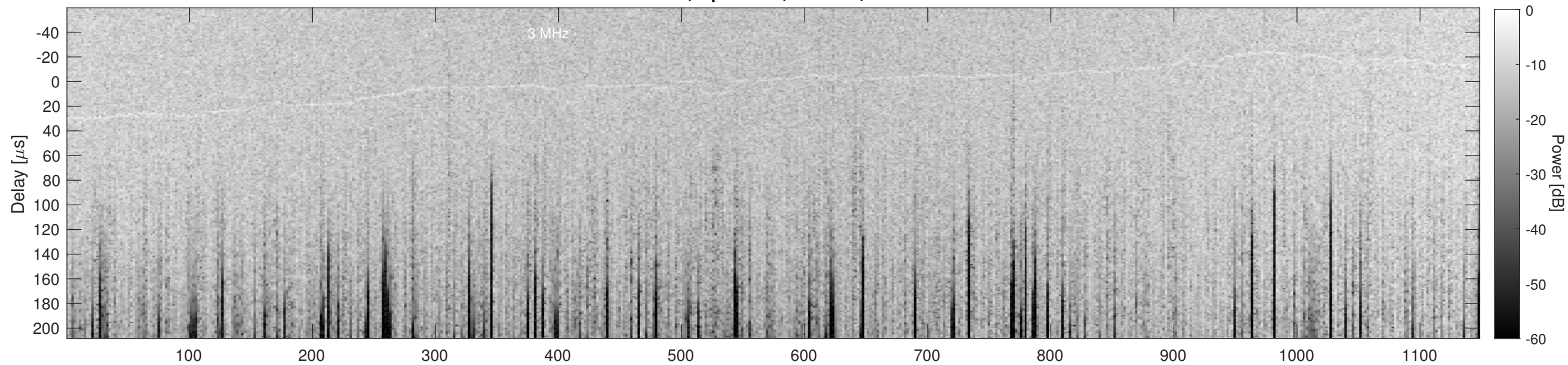
Orbit 15235, Cluttergram
