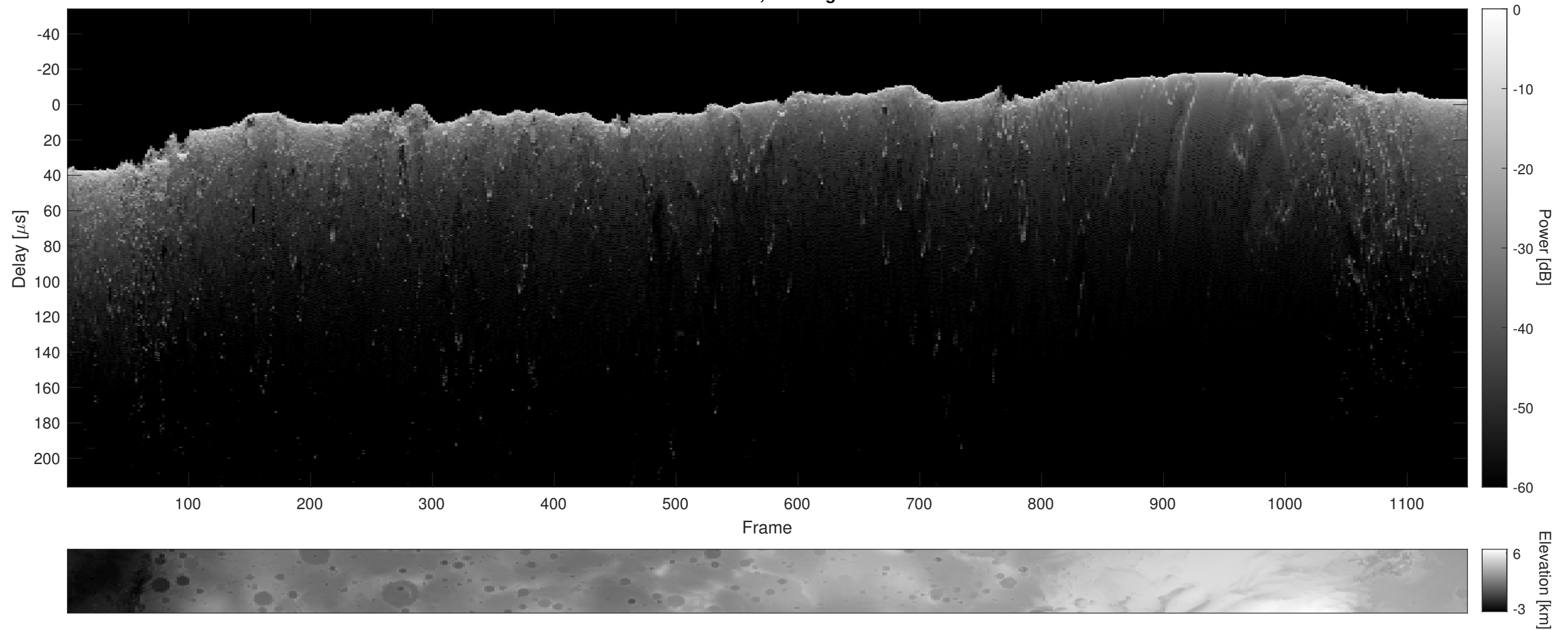
Orbit 15237, Cluttergram
