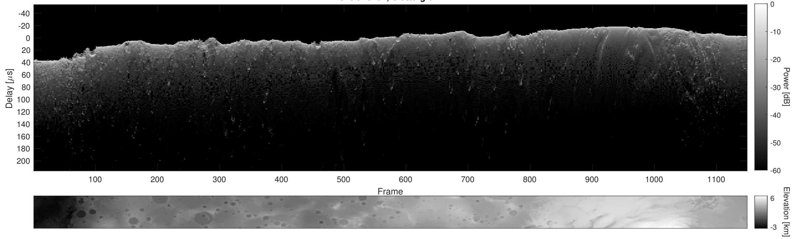
Orbit 15237, Cluttergram
