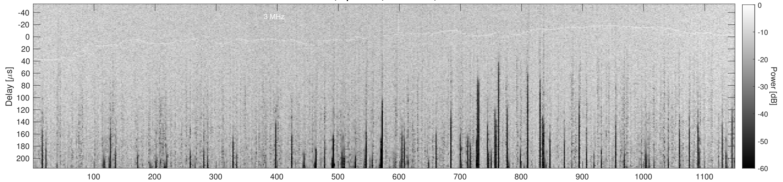
Orbit 15237, Cluttergram
