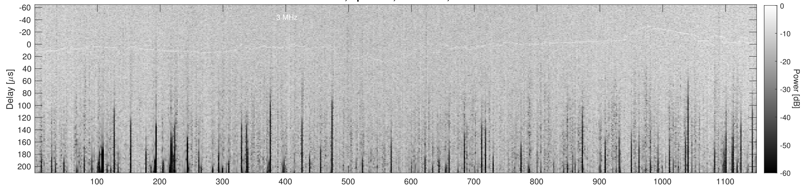
Orbit 15239, Cluttergram
