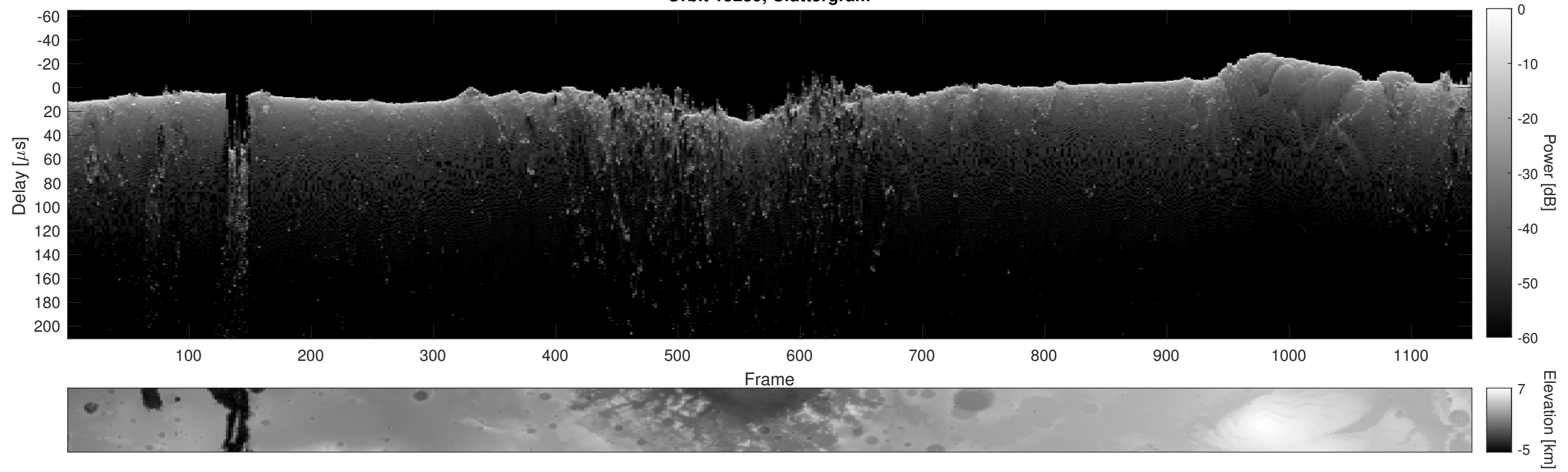
Orbit 15239, Cluttergram
