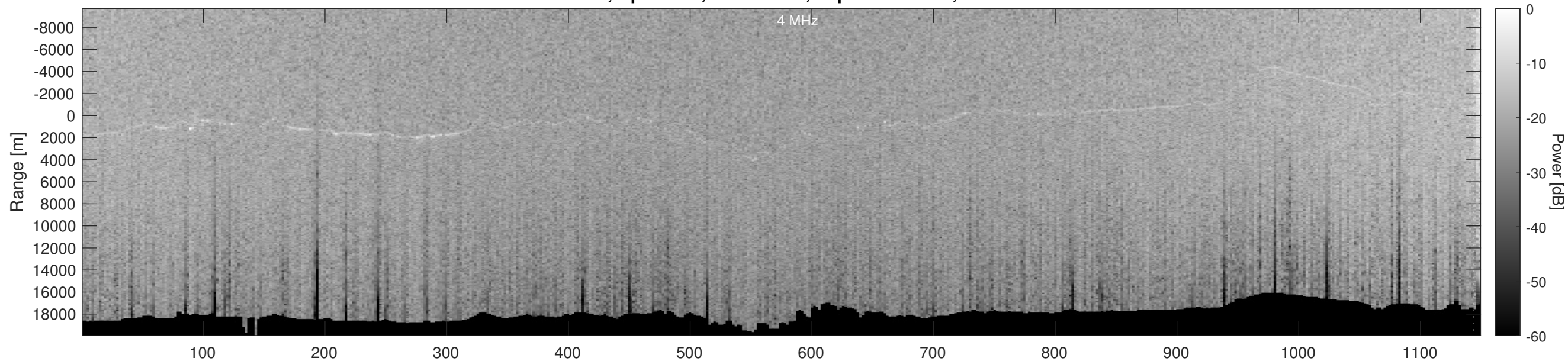
Orbit 15239, Optimized, No Window, Depth-Corrected, Channel 2
