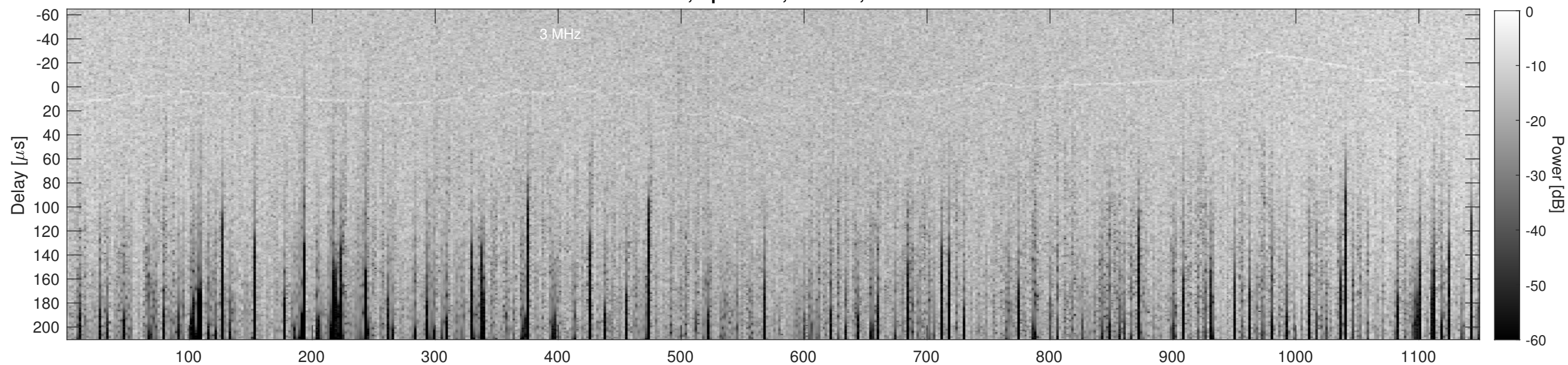
Orbit 15239, Cluttergram
