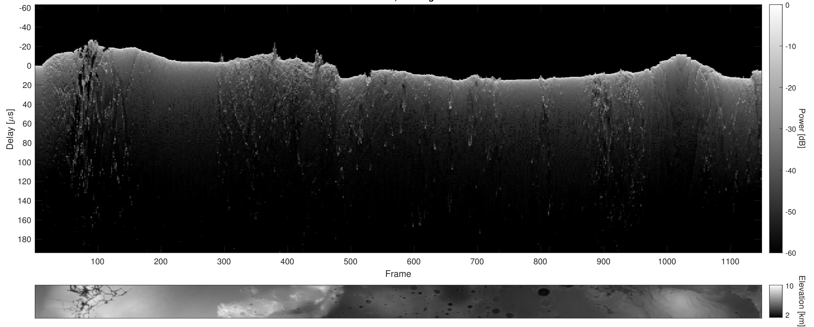
Orbit 15250, Cluttergram
