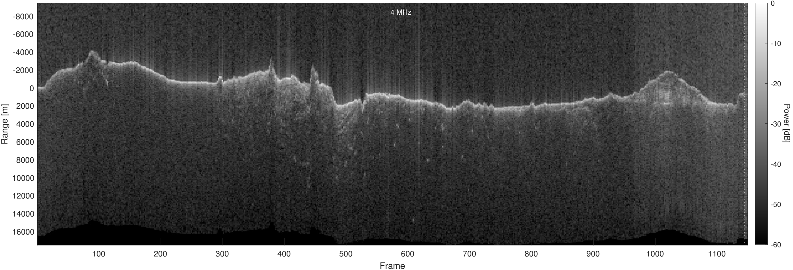
Orbit 15250, Optimized, No Window, Depth-Corrected, Channel 2
