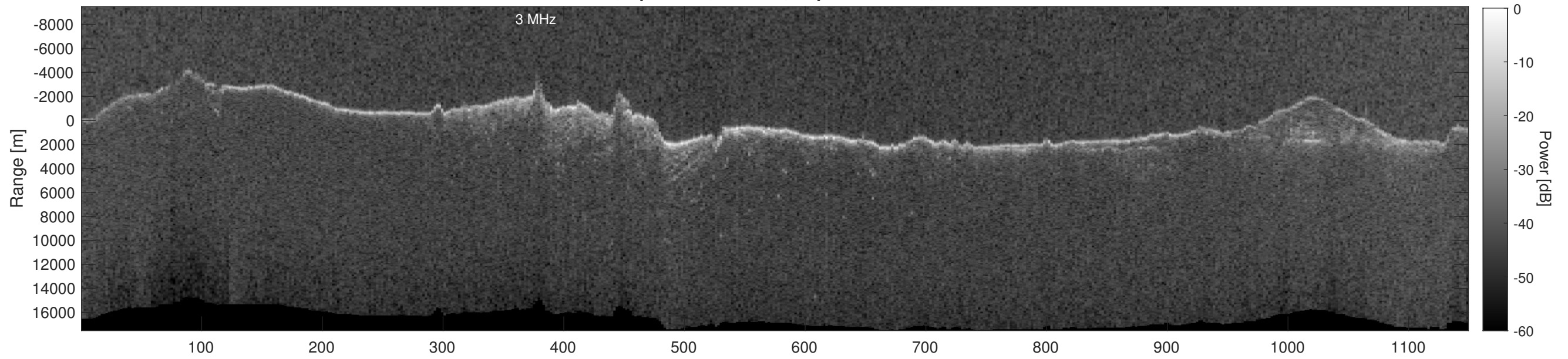
Orbit 15250, Depth-Corrected Cluttergram
