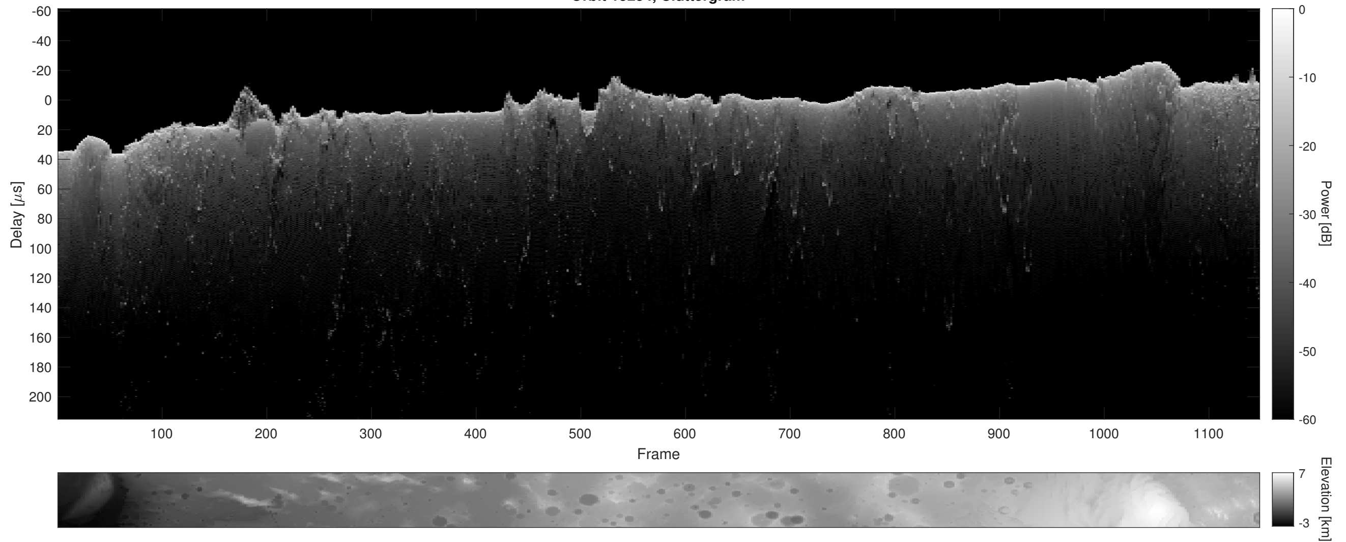
Orbit 15254, Cluttergram
