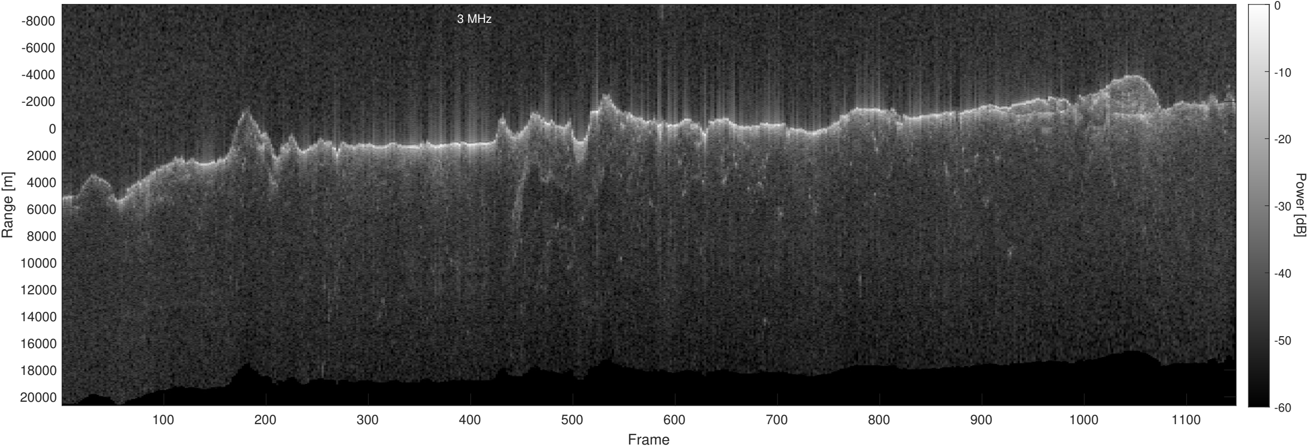
Orbit 15254, Optimized, No Window, Depth-Corrected, Channel 2
