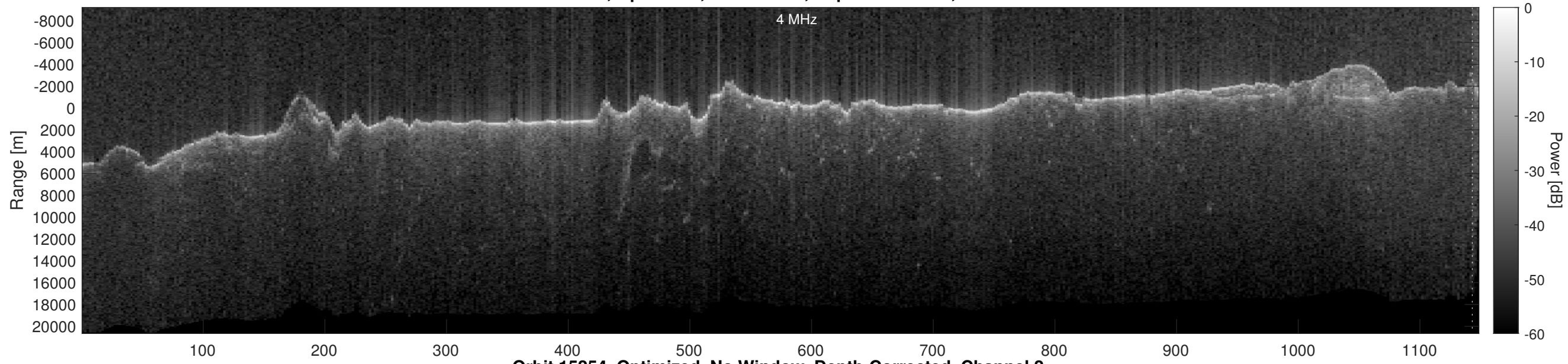
Orbit 15254, Optimized, No Window, Depth-Corrected, Channel 2
