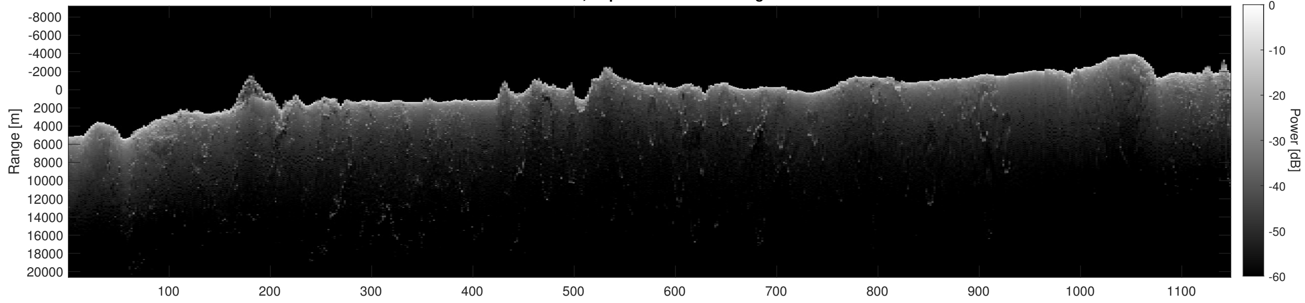
Orbit 15254, Depth-Corrected Cluttergram
