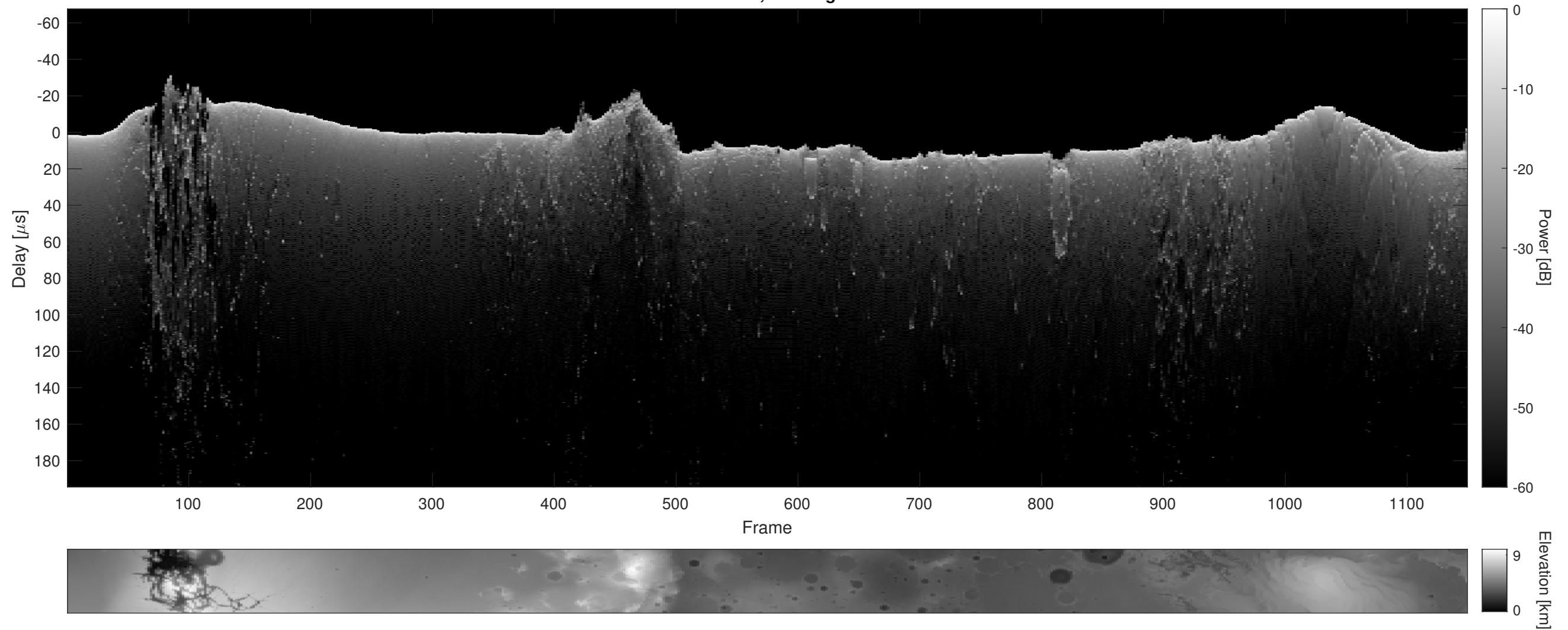
Orbit 15257, Cluttergram
