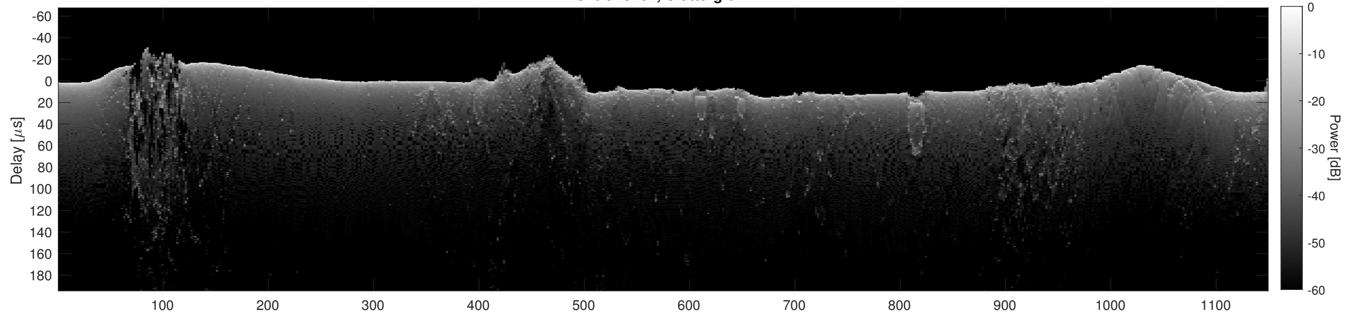
Orbit 15257, Cluttergram
