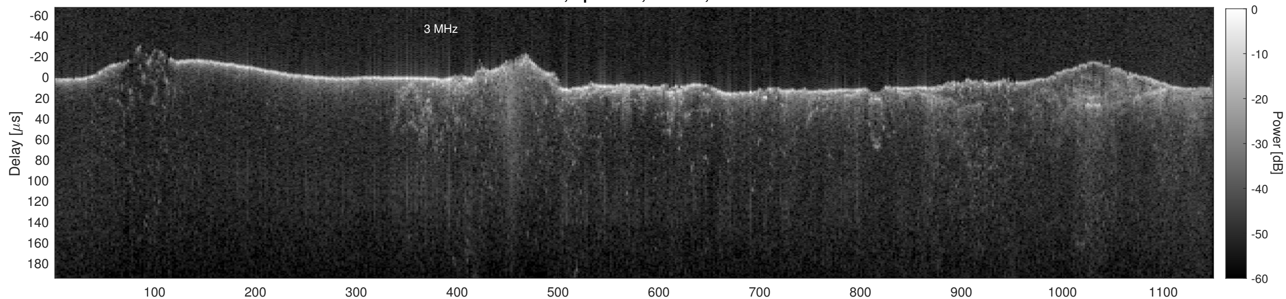
Orbit 15257, Cluttergram
