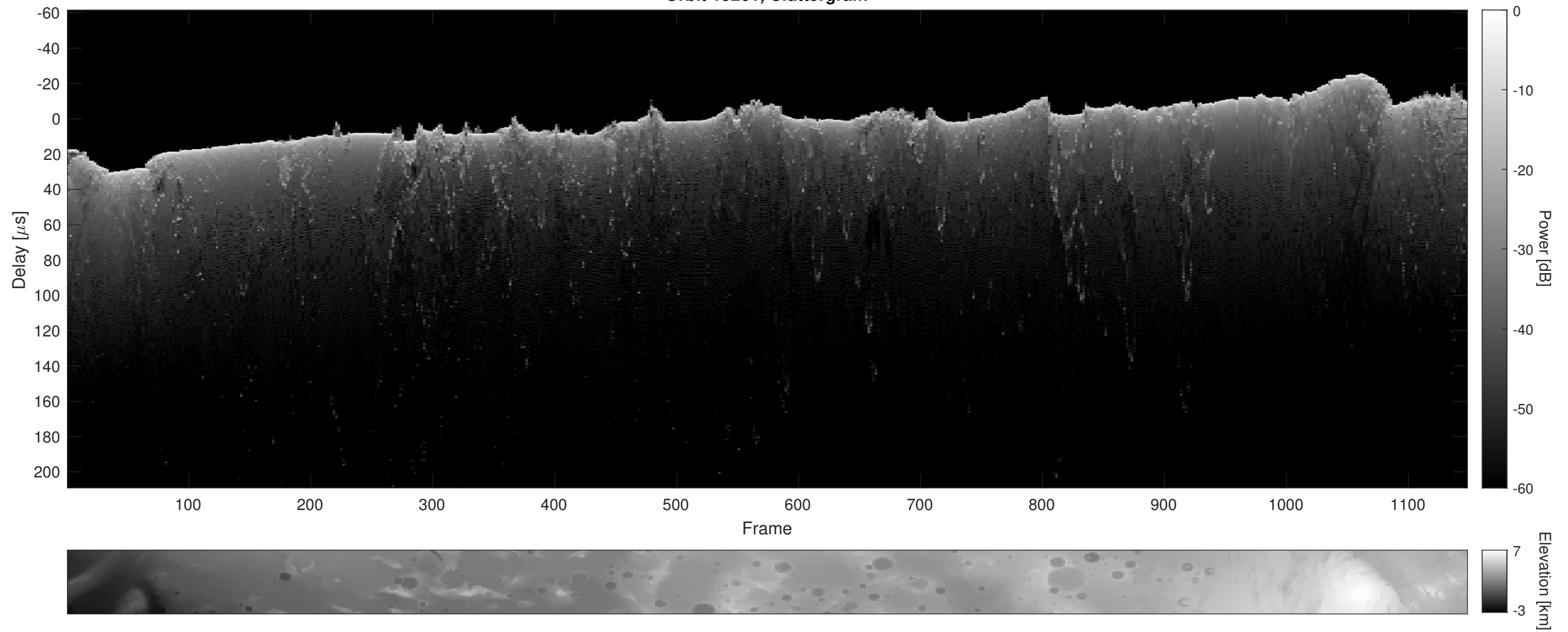
Orbit 15261, Cluttergram
