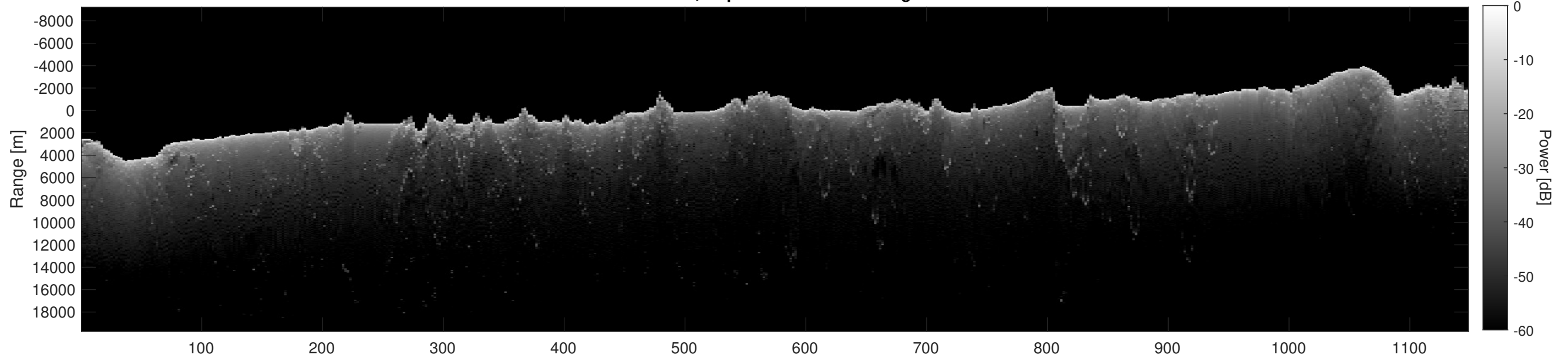
Orbit 15261, Depth-Corrected Cluttergram
