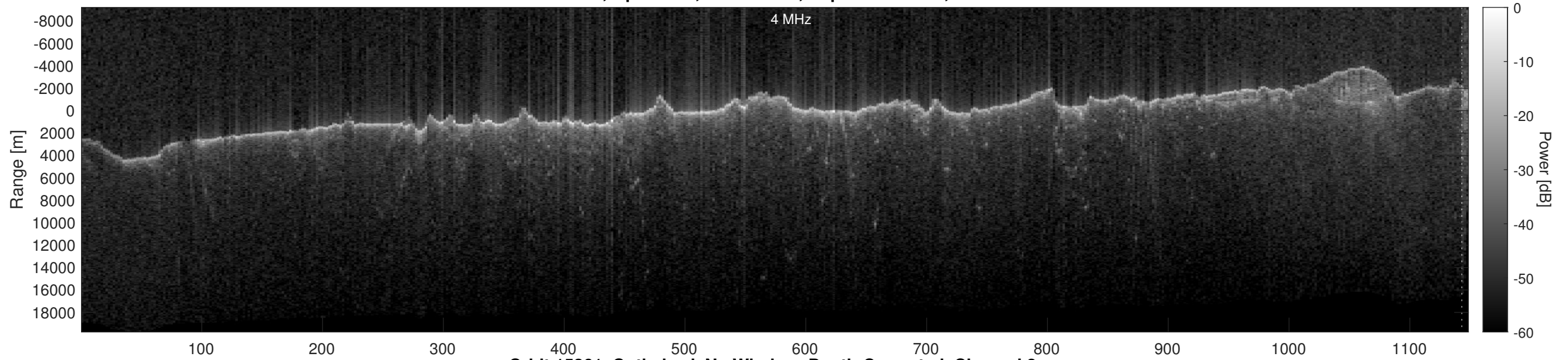
Orbit 15261, Optimized, No Window, Depth-Corrected, Channel 2
