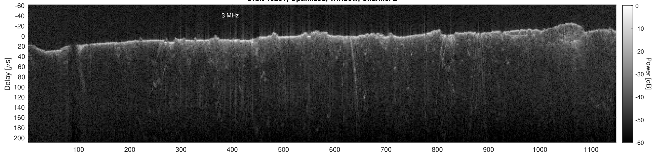
Orbit 15261, Cluttergram
