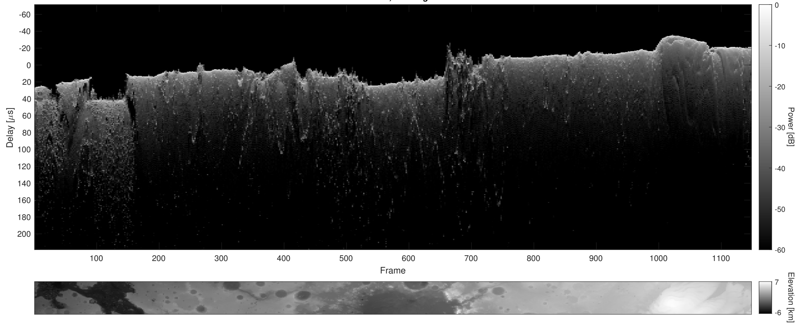
Orbit 15267, Cluttergram
