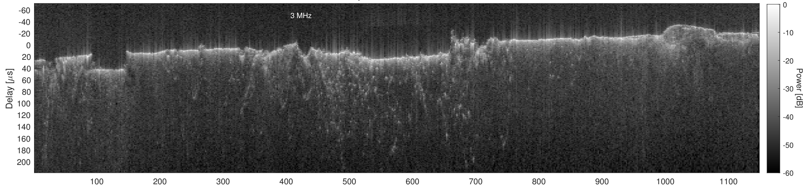
Orbit 15267, Cluttergram
