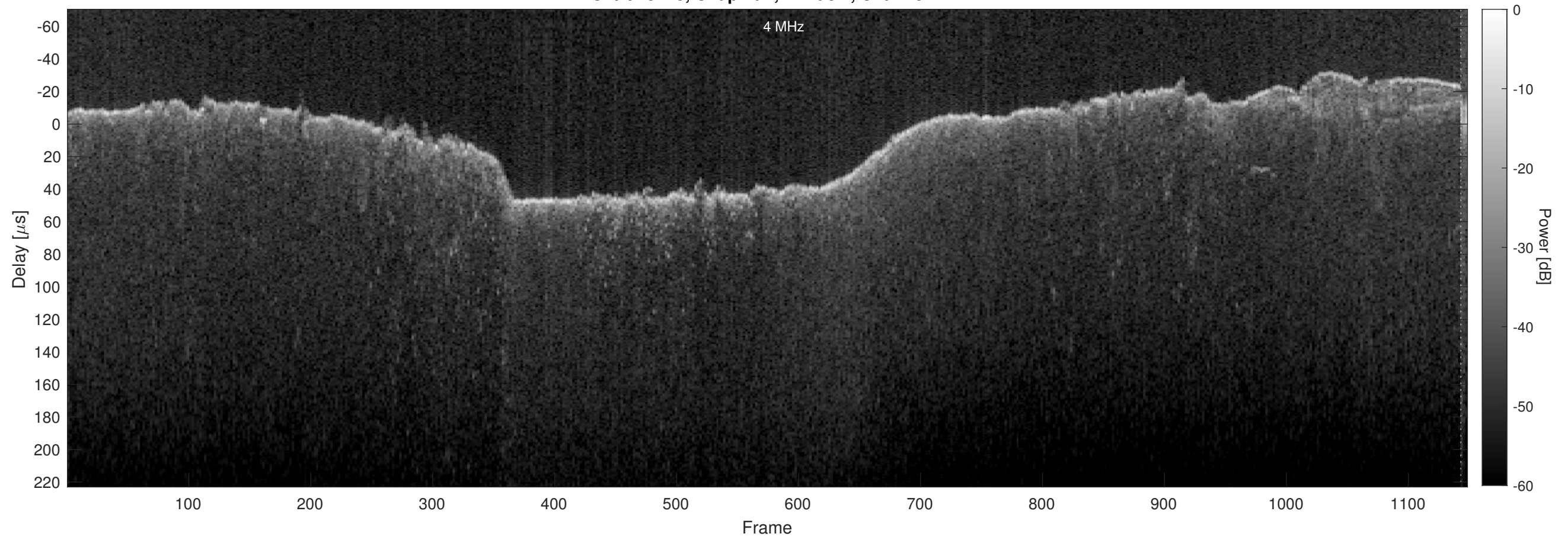
Orbit 15273, Chapman, Window, Channel 2
