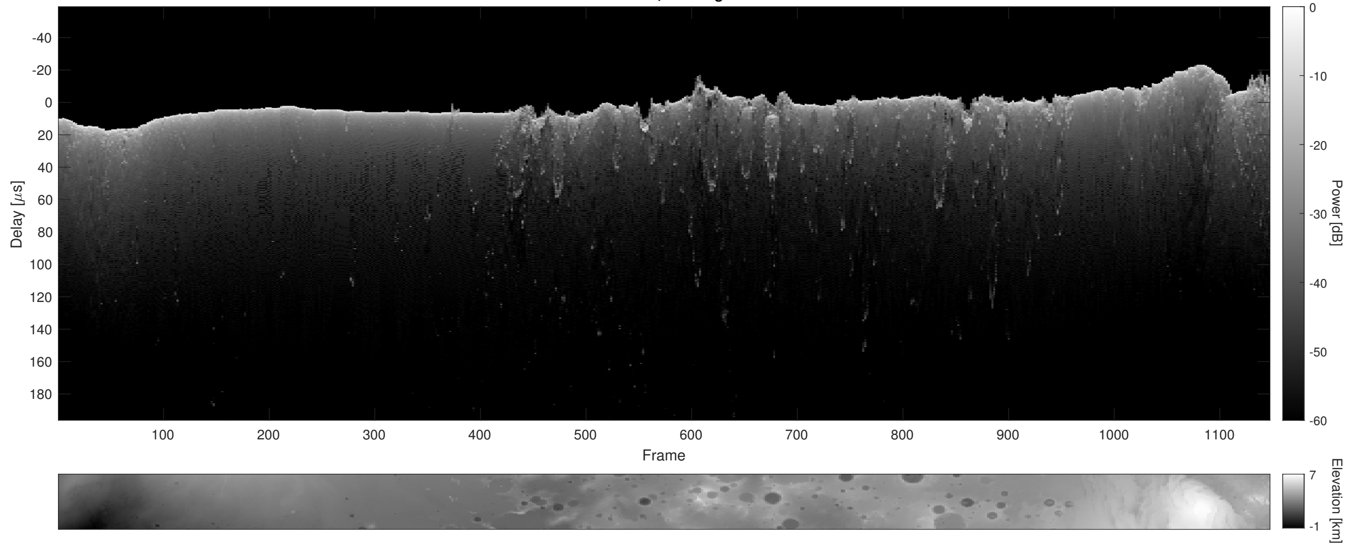
Orbit 15275, Cluttergram
