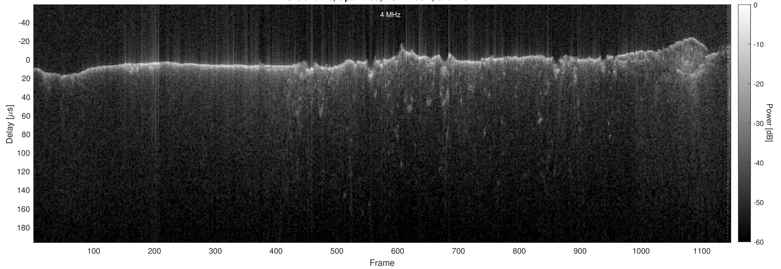
Orbit 15275, Optimized, No Window, Channel 2
