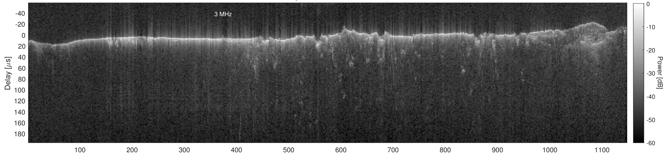
Orbit 15275, Cluttergram
