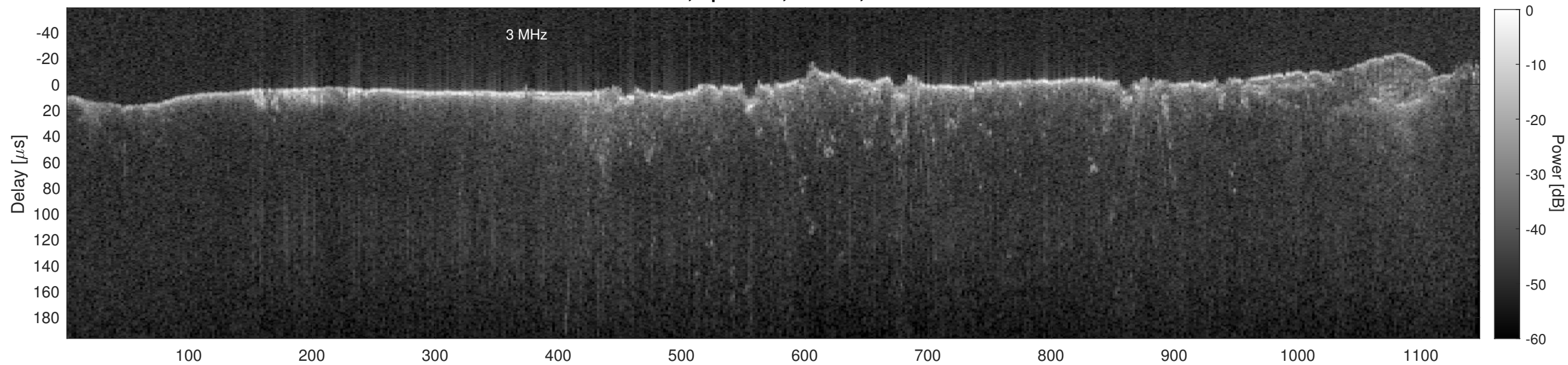
Orbit 15275, Cluttergram
