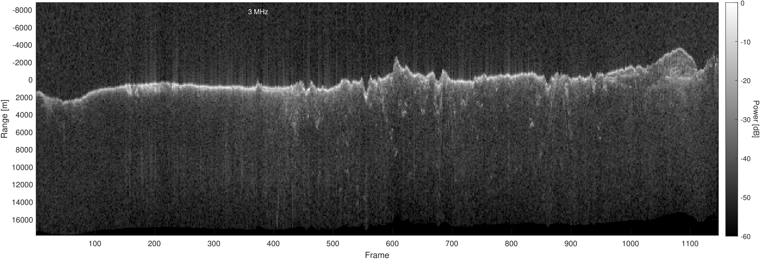
Orbit 15275, Optimized, Window, Depth-Corrected, Channel 2
