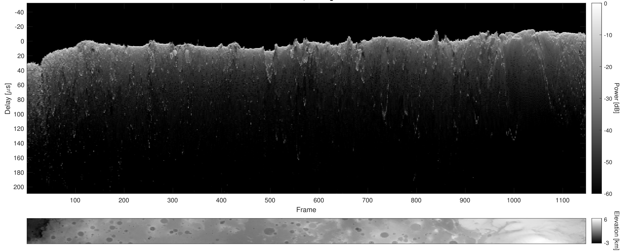
Orbit 15276, Cluttergram
