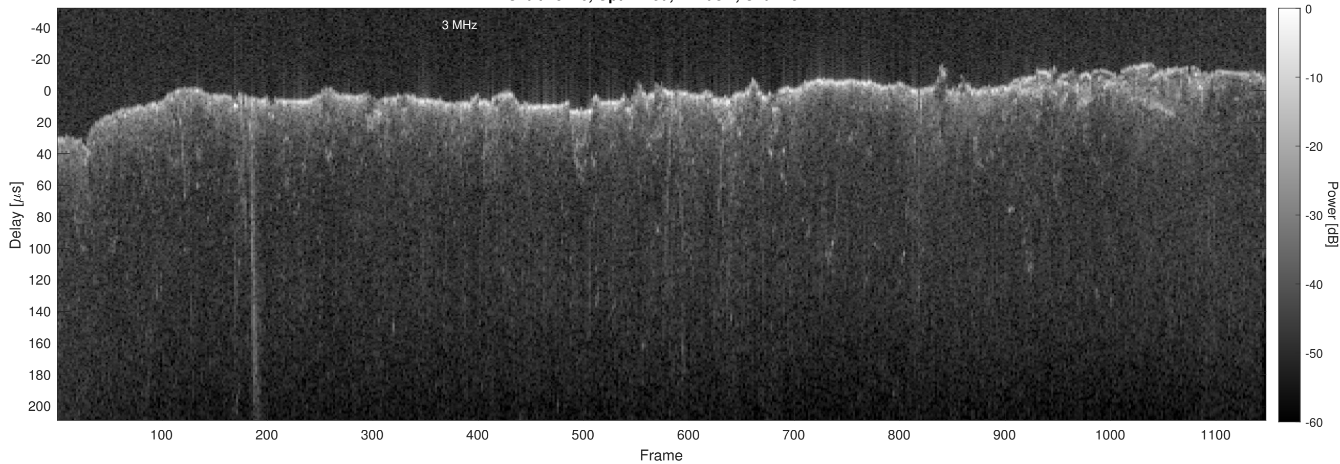
Orbit 15276, Optimized, Window, Channel 2
