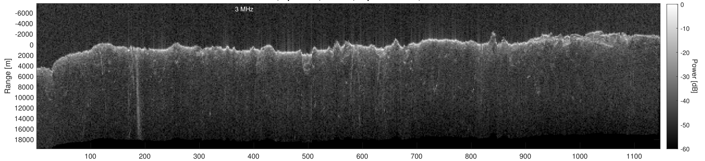
Orbit 15276, Depth-Corrected Cluttergram
