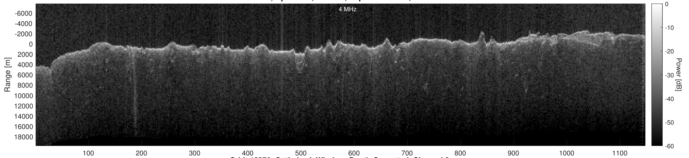
Orbit 15276, Optimized, Window, Depth-Corrected, Channel 2
