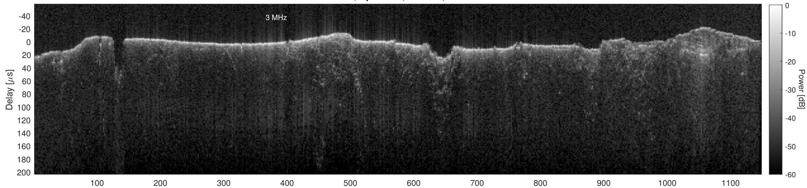
Orbit 15278, Cluttergram
