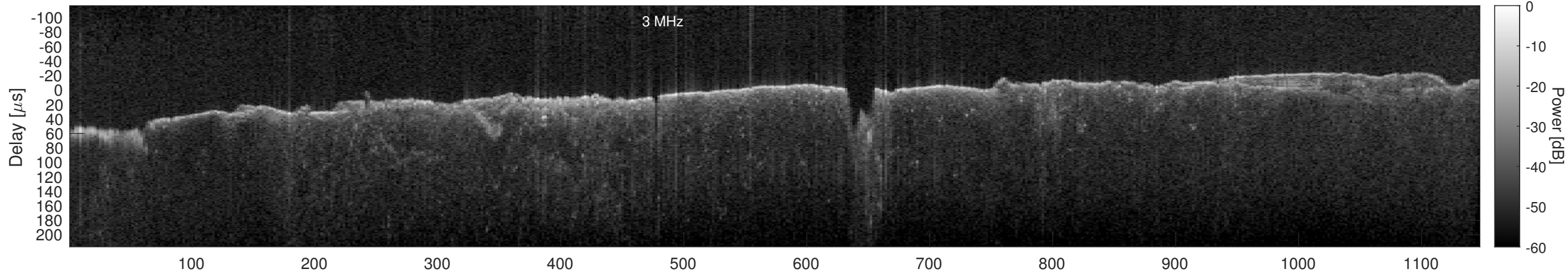
Orbit 15279, Window, Channel 2, Chapman
