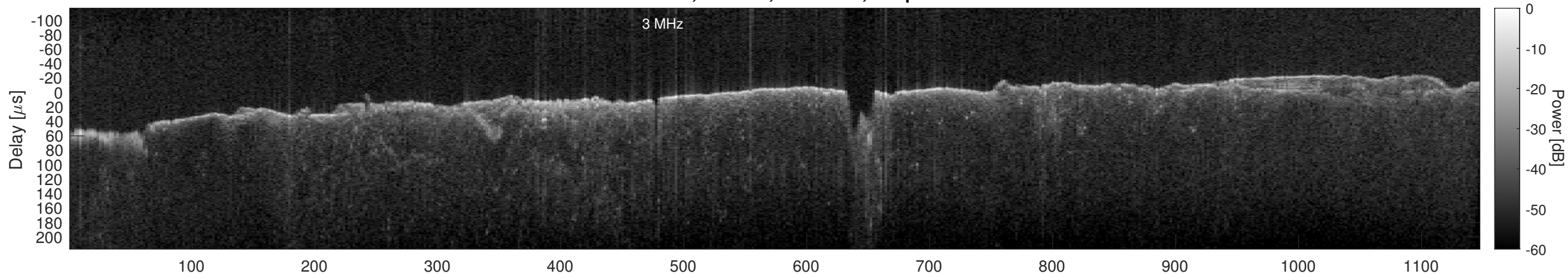
Orbit 15279, Window, Channel 2, Optimized
