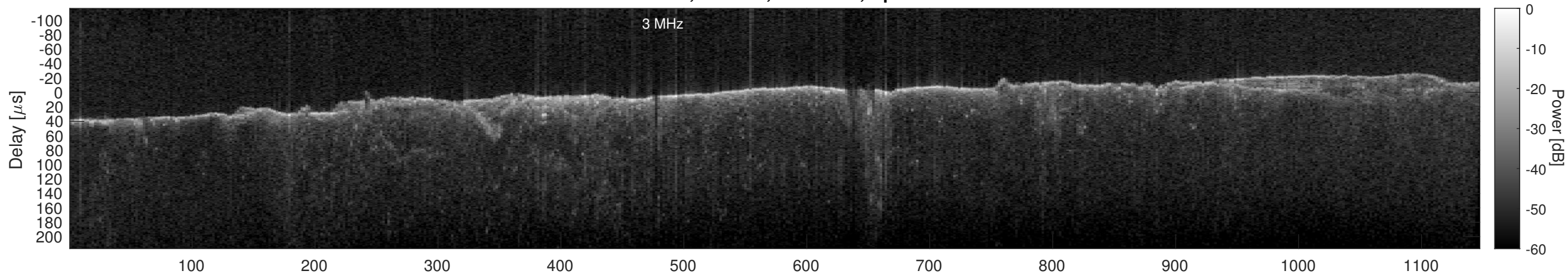
Orbit 15279, Cluttergram
